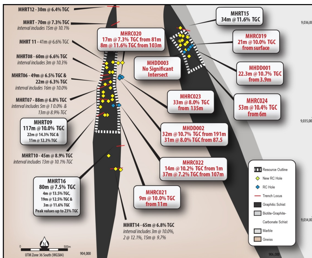
Figure 1 – Location plan of the Epanko deposit
