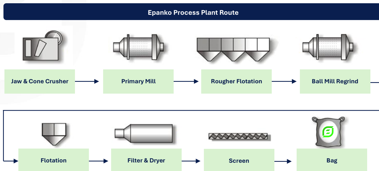
Figure 2: Epanko Process Plant Route
