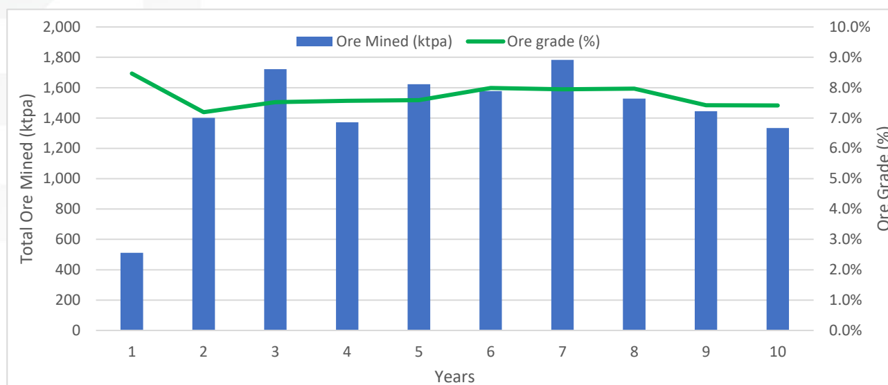
Figure 1: Total ore mined and ore grade for 20% increase in production rate (first 10 years)
