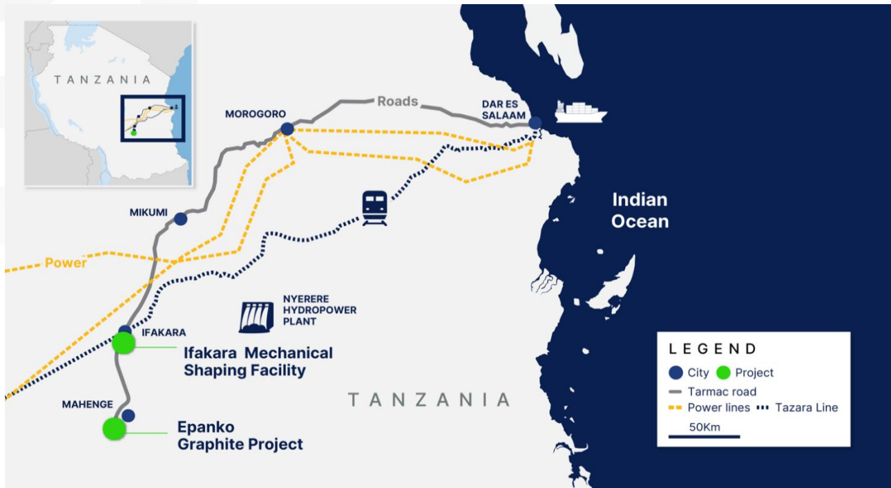
Figure 4: Epanko Site Location & Infrastructure
